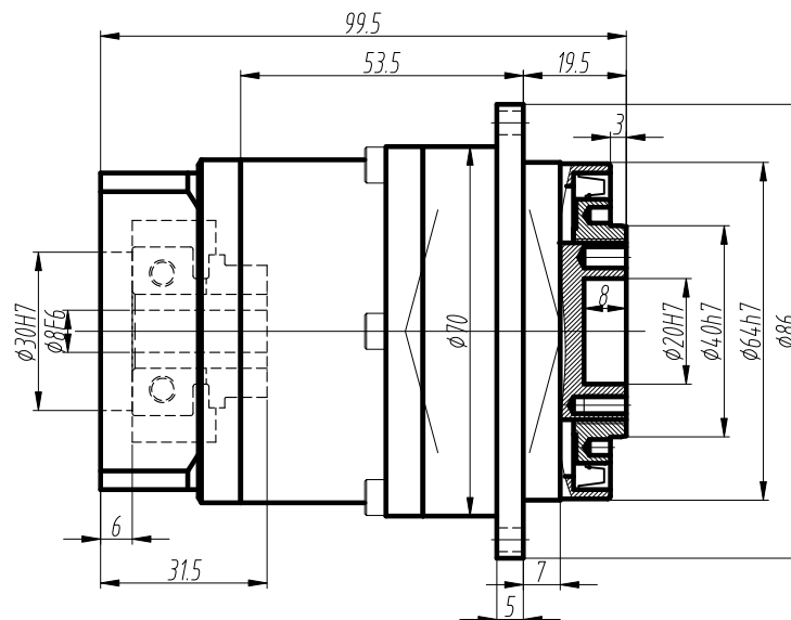
标准轴 Standard output shaft
